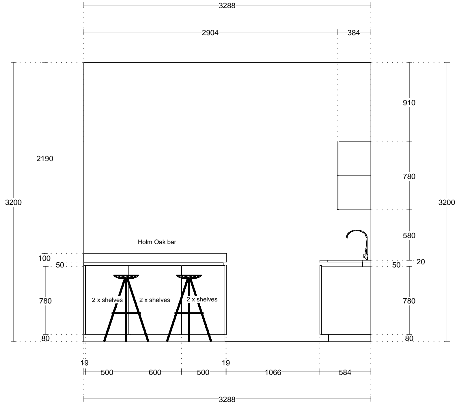
ELEVATION D
